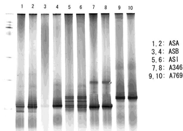
Fig. 1: DGGE of contaminants in jet fuel.
